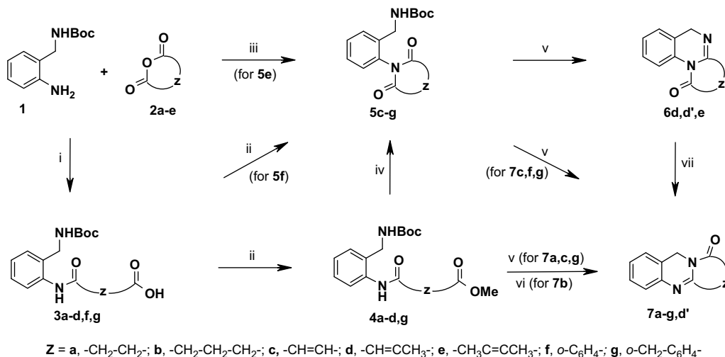
Scheme 1. General theme for synthesis of linear and angular 1,3-diaza-heterocycles. Reagents and conditions: (i) Et 2 O, 0 °C to rt, 3 h; (ii) CH 2 N 2 , Et 2 O, 0 °C, 30 min; (iii) EtOH, reflux, 1 h; (iv) Et 3 N, DCM, rt, 5 h; (v) TFA, DCM, rt, 5 h; (vi) TFA, DCM, rt, 5 h then MeOH, reflux, 5 h; (vii) AcOH, MeOH, reflux, 24/48 h.
