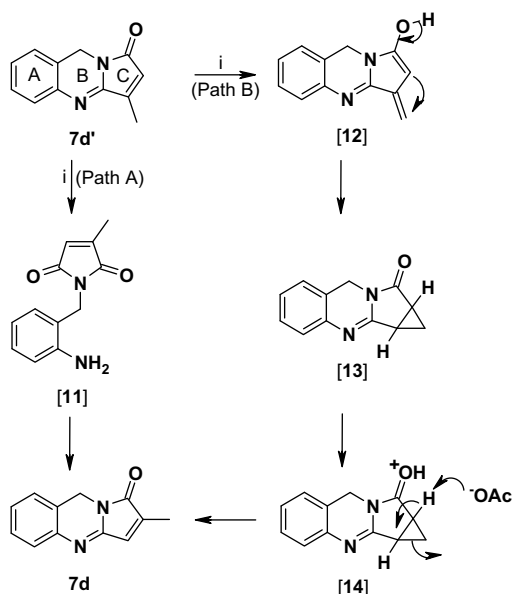
Scheme 2. Proposed mechanisms for the observed 1,2-methyl shift. Reaction condition: (i) AcOH/MeOH, reflux, 15 days (96%).
